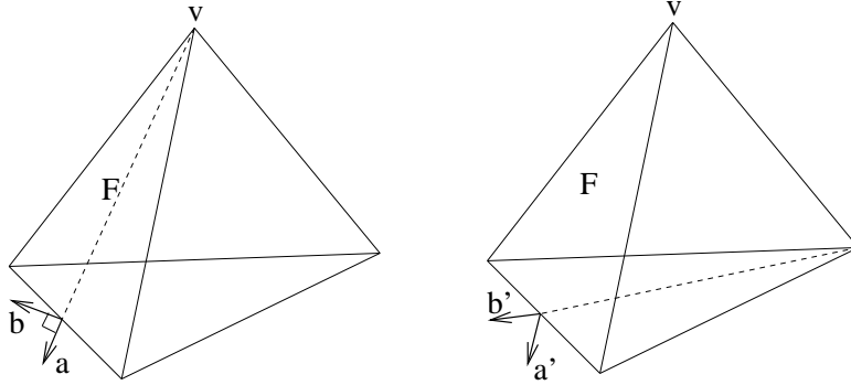
FIGURE 1. The vectors a , b , a' and b'
