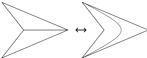
FIGURE 1. A 2-2 combinatorial bistellar move which is not geometric.
